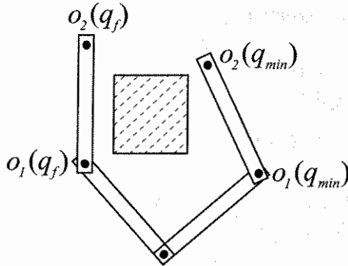
Figure 5.9: The configuration q_{\min} is a local minimum in the potential field. At q_{\min} the attractive force exactly cancels the repulsive force and the planner fails to make further progress.
