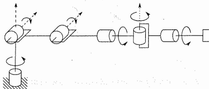
Figure 3.29: Elbow manipulator with spherical wrist.
