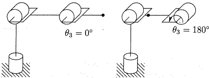
Figure 4.6: Elbow singularities of the elbow manipulator.
