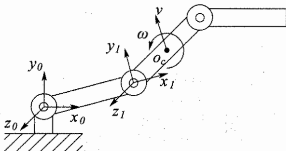
Figure 4.3: Finding the velocity of link 2 of a 3-link planar robot.
