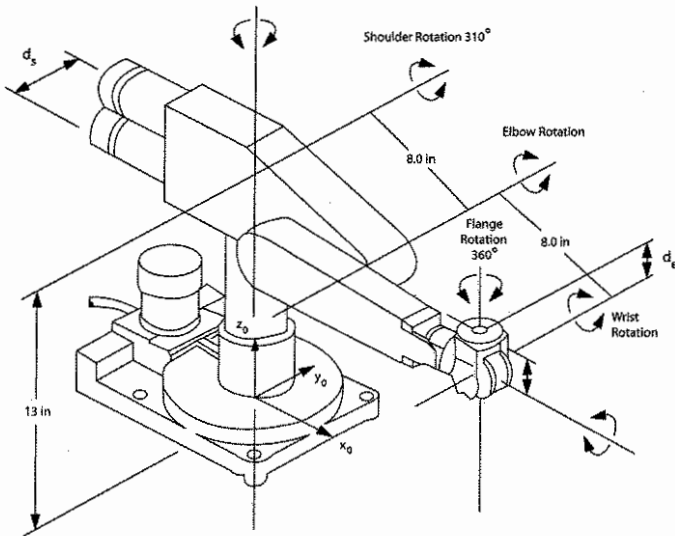
Figure 3.31: PUMA 260 manipulator.
