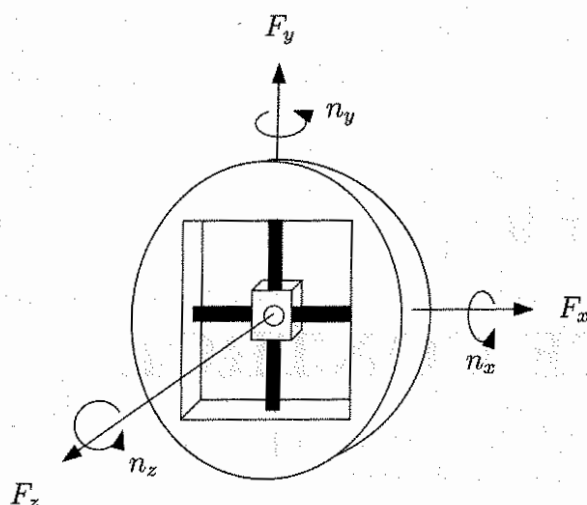
Figure 9.1: A wrist force sensor.
