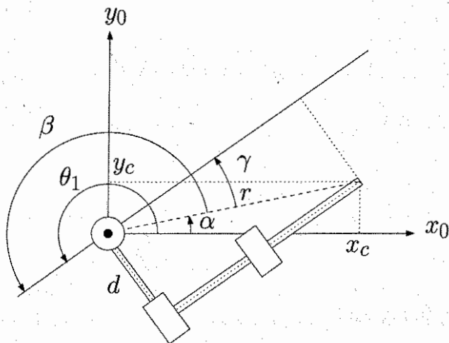
Figure 3.18: Right arm configuration.
