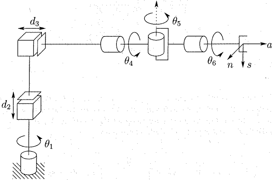
Figure 3.9: Cylindrical robot with spherical wrist.
