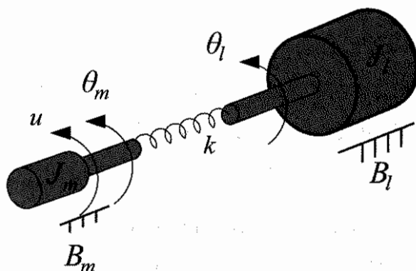
Figure 6.20: Idealized model to represent joint flexibility. The stiffness constant k represents the effective torsional stiffness of the harmonic drive.
