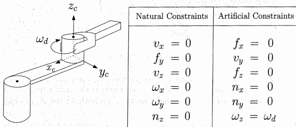
Figure 9.4: Turning a crank.
