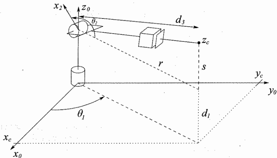
Figure 3.21: Spherical manipulator.
