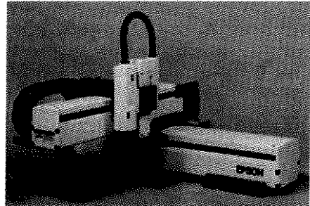
Figure 1.16: The Epson Cartesian Robot. Cartesian robot designs allow increased structural rigidity and hence higher precision. Cartesian robots are often used in pick and place operations. (Photo courtesy of Epson Robots.)
