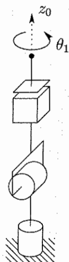
Figure 4.9: Singularity of spherical manipulator with no offsets.
