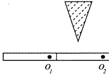
Figure 5.6: The repulsive forces exerted on the origins of the DH frames o_1 and o_2 may not be sufficient to prevent a collision between link 2 and the obstacle.
