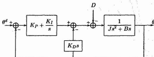
Figure 6.12: Closed-loop system with PID control. The integrator added to the compensator increases the system order from two to three and increases the system type number from 1 to 2.
