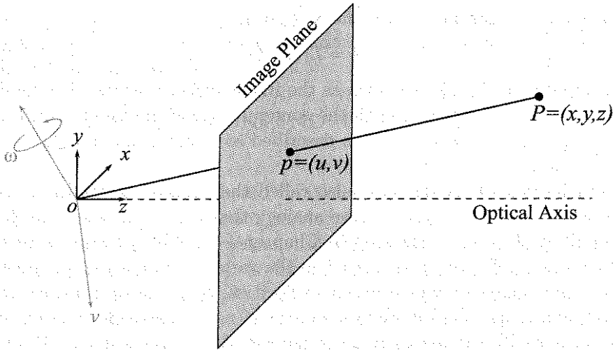
Figure 12.1: The point P is fixed with respect to the world coordinate frame, and the camera frame moves with angular velocity \omega and linear velocity v .
