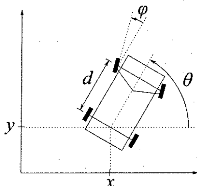
Figure 10.7: The kinematic car.
