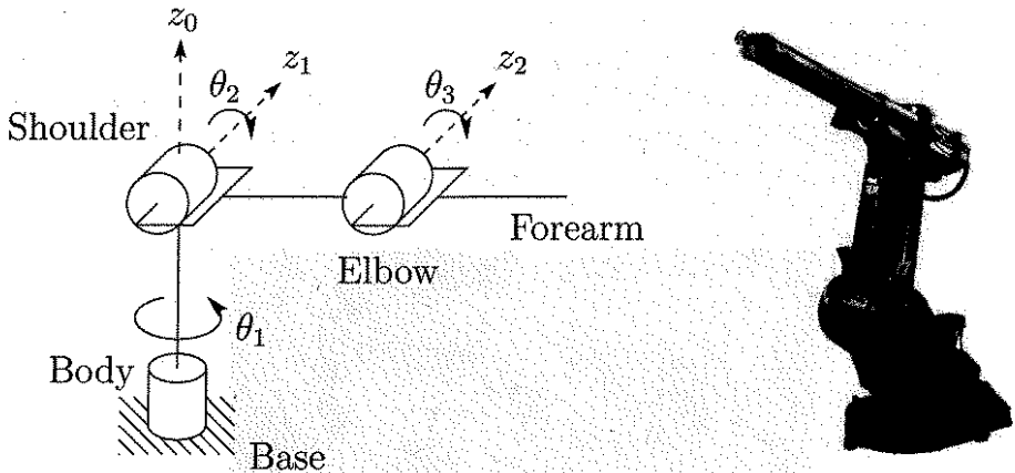
Figure 1.9: The ABB IRB1400 Robot, a six-DOF elbow manipulator (right). The symbolic representation of this manipulator (left) shows why it is referred to as an anthropomorphic robot. The links and joints are analogous to human joints and limbs. (Photo courtesy of ABB.)
