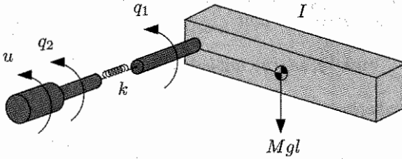
Figure 10.5: Single-link, flexible joint robot.
