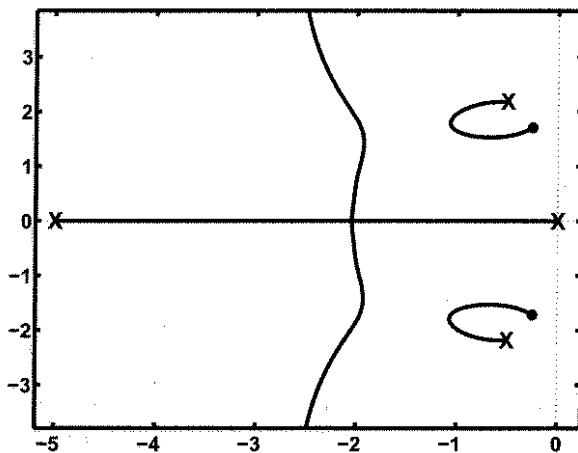
Figure 6.23: Root locus for the system of Figure 6.22.
