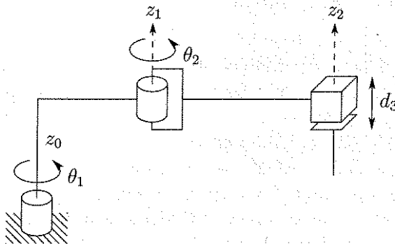
Figure 1.13: Symbolic representation of the SCARA arm.
