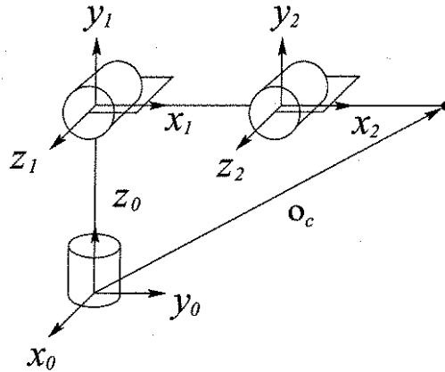
Figure 4.5: Elbow manipulator.
