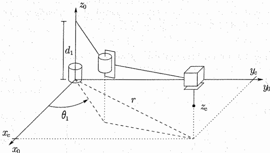
Figure 3.22: SCARA manipulator.
