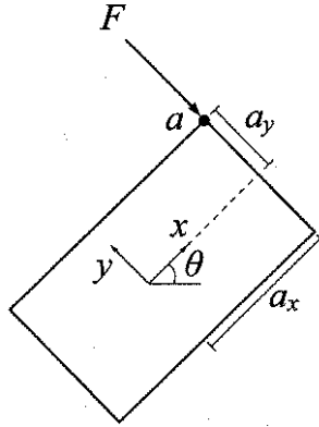
Figure 5.7: In this example, the robot is a polygon whose configuration can be represented as q = (x, y, \theta) , in which \theta is the angle from the world x -axis to the x -axis of the robot's local frame. A force F is exerted on vertex a with local coordinates (a_x, a_y) .
