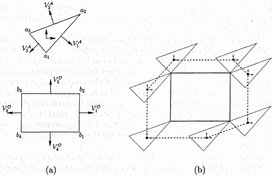
Figure 5.1: (a) The robot end effector is a triangle-shaped rigid object in a workspace that contains a single rectangular obstacle. (b) The boundary of the configuration space obstacle QO (shown as a dashed line) can be obtained by computing the convex hull of the configurations at which the end effector makes vertex-to-vertex contact with the single convex obstacle.
