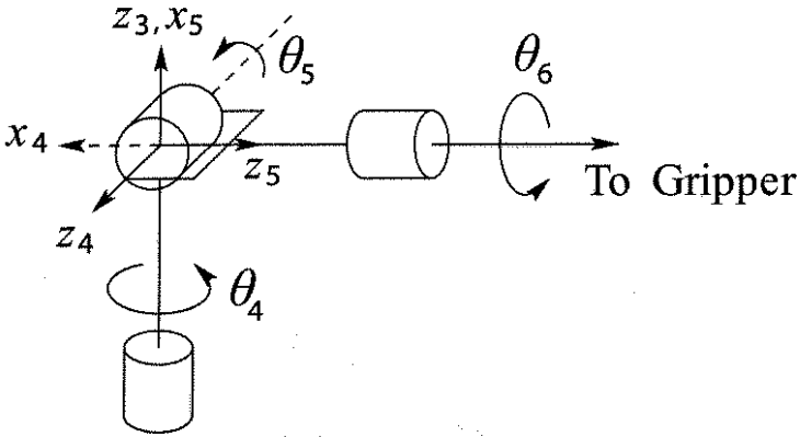
Figure 3.8: The spherical wrist frame assignment.
