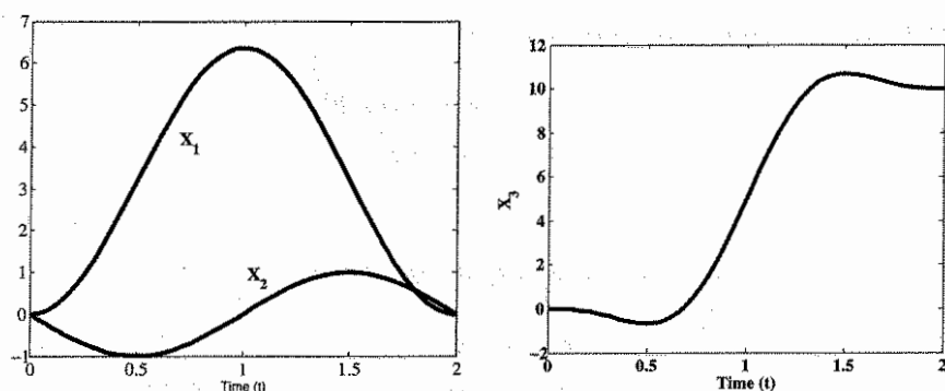
Figure 10.10: Response of x_1 , x_2 and x_3 . Note that x_1 and x_2 return to their original values after 2 seconds while x_3 moves from the origin to x_3 = 10 as desired.
