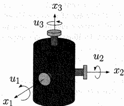
Figure 10.9: Satellite with reaction wheels.
