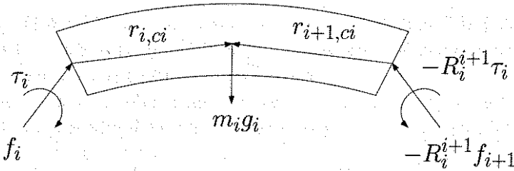
Figure 7.12: Forces and moments on link i .
