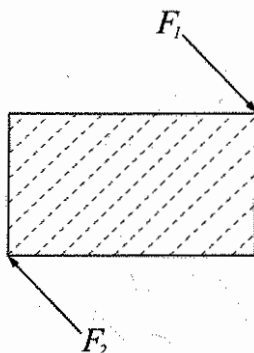
Figure 5.8: This example illustrates why forces must be mapped to the configuration space before they are combined. The two forces illustrated in the figure are vectors of equal magnitude in opposite directions. Vector addition of these two forces produces zero net force, but there is a net torque induced by these forces.
