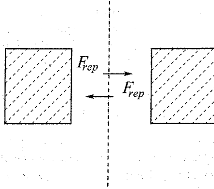
Figure 5.5: In this case the gradient of the repulsive potential given by Equation (5.6) is not continuous. In particular, the gradient changes discontinuously when o_i crosses the line midway between the two obstacles.
