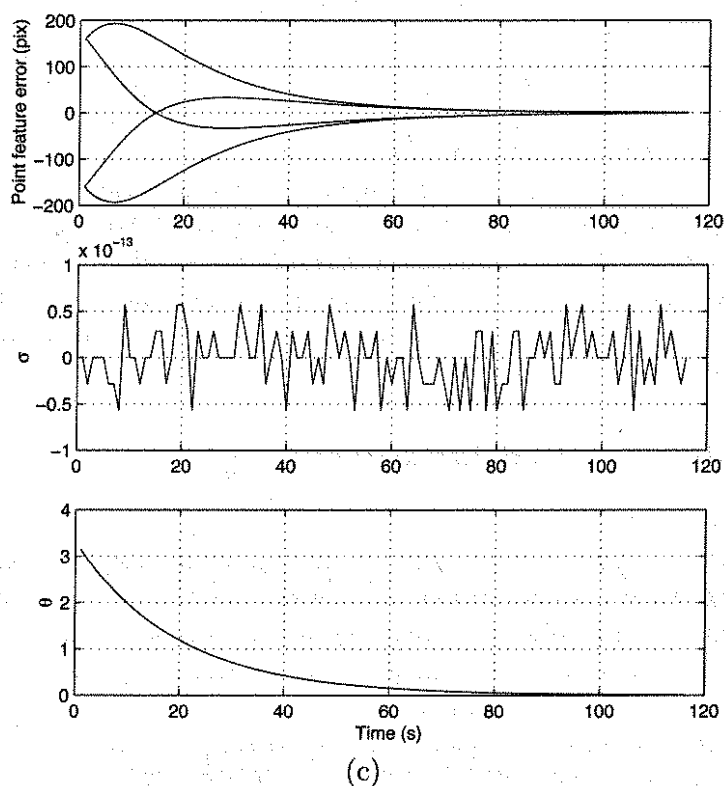
Figure 12.4: Partitioned method for pure target rotation ( \pi rad). (a) Image-plane feature motion with initial location denoted by \circ and desired location denoted by \bullet . (b) Cartesian translation trajectory. (c) Feature error trajectory.
