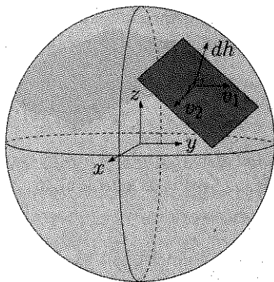
Figure 10.1: The sphere as a two-dimensional manifold in \mathbb{R}^3 .
