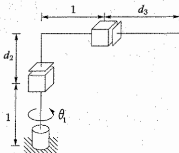
Figure 3.34: Cylindrical configuration.
