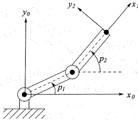
Figure 7.10: Generalized coordinates for the robot of Figure 6.4.
