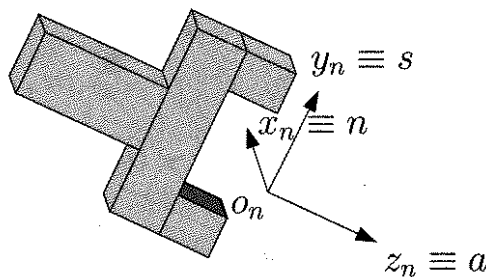
Figure 3.5: Tool frame assignment.
