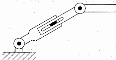
Figure 3.33: Three-link planar robot with prismatic joint.
