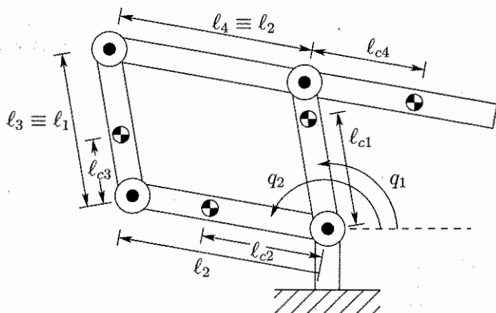
Figure 7.11: Five-bar linkage.
