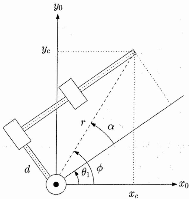
Figure 3.17: Left arm configuration.
