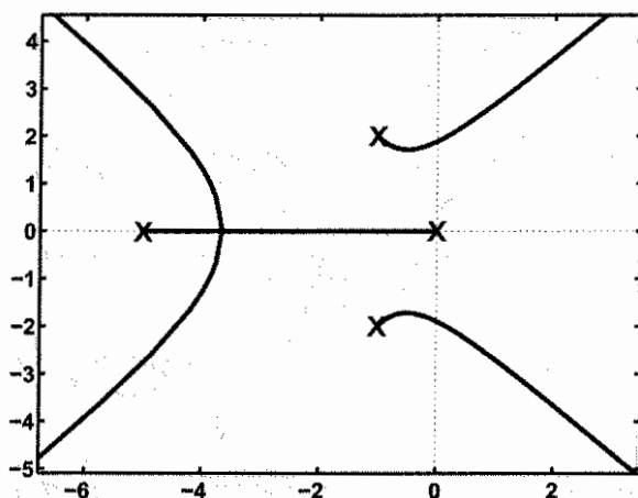
Figure 6.25: Root locus for the system of Figure 6.24.
