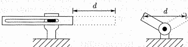
Figure 1.5: Linear vs. rotational link motion showing that a smaller revolute joint can cover the same distance d as a larger prismatic joint. The tip of a prismatic link can cover a distance equal to the length of the link. The tip of a rotational link of length a , by contrast, can cover a distance of 2a by rotating 180 degrees.
