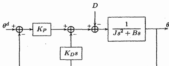
Figure 6.8: The system with PD control.
