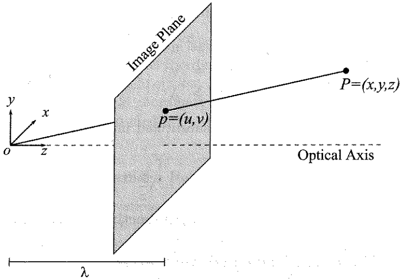
Figure 11.1: Camera coordinate frame.
