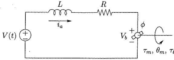
Figure 6.3: Circuit diagram for an armature controlled DC motor. The rotor windings have an effective inductance L and resistance R . The applied voltage V is the control input.
