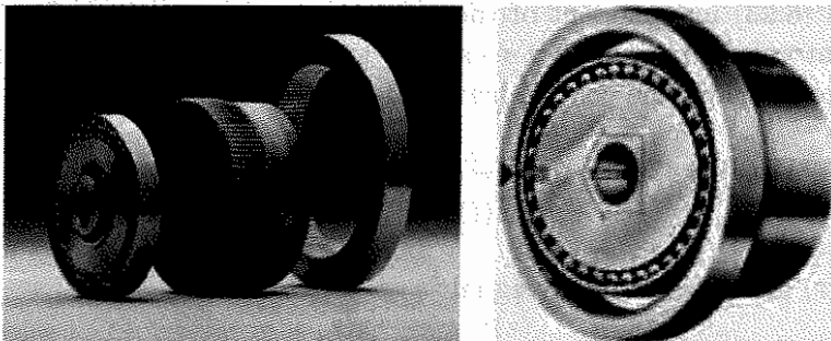
Figure 6.19: The harmonic drive. The rotation of the elliptical wave generator meshes the teeth of the flexspline and circular spline resulting in low backlash and high torque transmission. (Courtesy of HD Systems, www.hdsi.net .)
