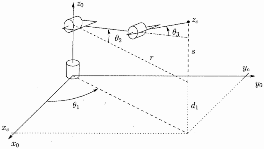
Figure 3.13: Elbow manipulator.
