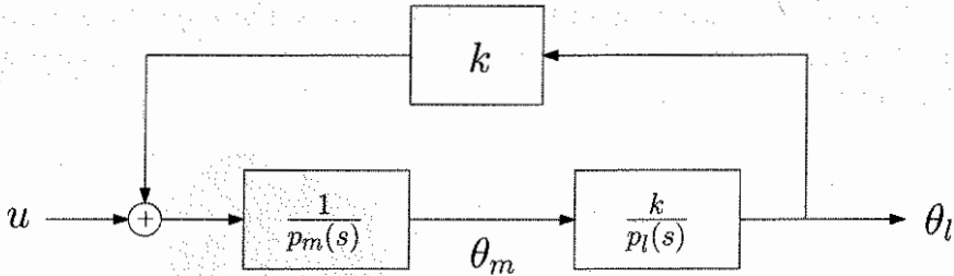
Figure 6.21: Block diagram for the system (6.41) and (6.42).
