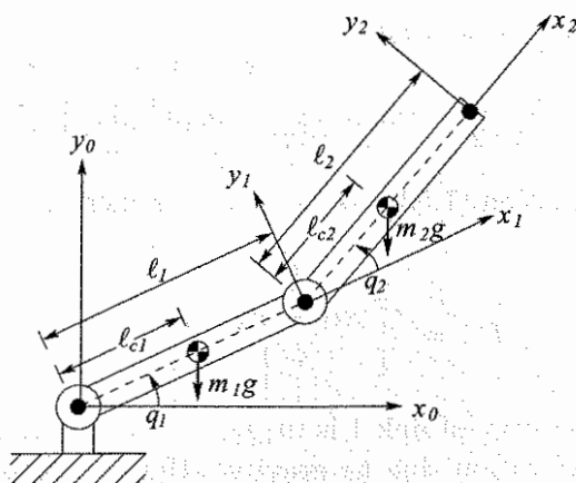
Figure 7.8: Two-link revolute joint arm. The rotational joint motion introduces dynamic coupling between the joints.
