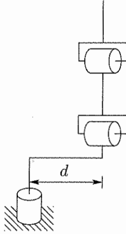
Figure 3.16: Elbow manipulator with shoulder offset.
