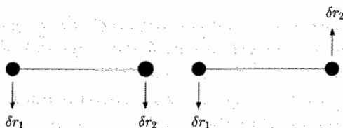
Figure 7.4: Examples of virtual displacements for a rigid bar. These infinitesimal motions do not change the distance between the endpoints and are thus compatible with the assumption that the bar is rigid.
