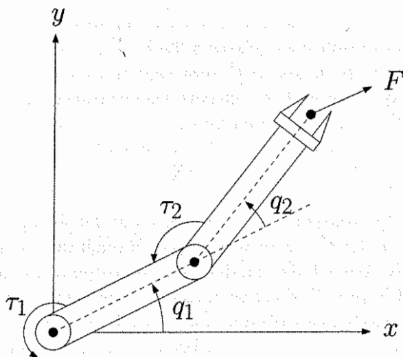
Figure 4.11: Two-link planar robot.
