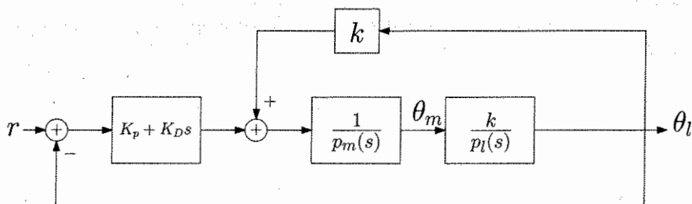
Figure 6.24: PD control with load angle feedback.
