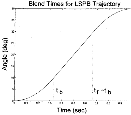
Figure 5.15: Blend times for LSPB trajectory.
