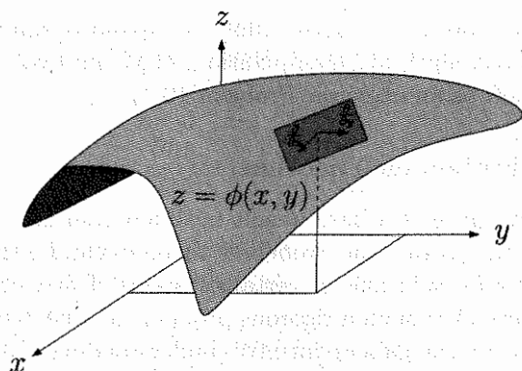
Figure 10.3: Integral manifold in \mathbb{R}^3 .
