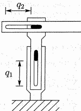
Figure 7.7: Two-link planar Cartesian robot. The orthogonal joint axes and linear joint motion of the Cartesian robot result in simple kinematics and dynamics.
