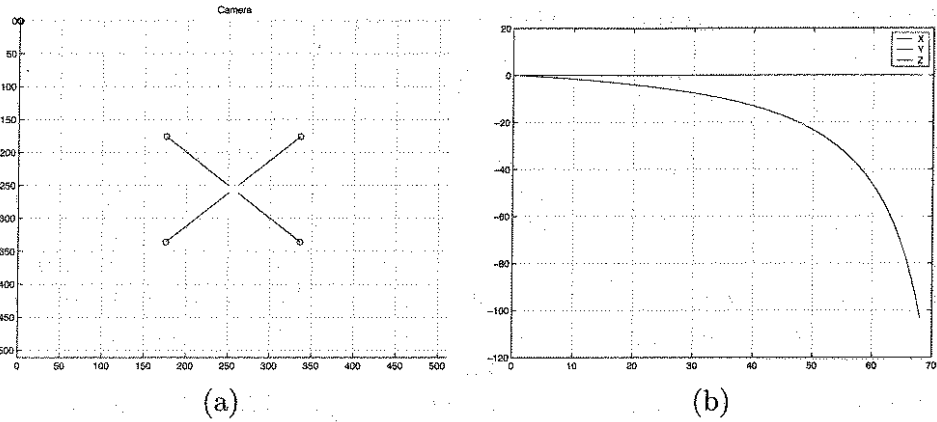
Figure 12.3: The required camera motion is a rotation by \pi about the camera z -axis. In (a) the feature points move along straight line trajectories in the image, but in (b) this requires the camera to retreat to z = -\infty .
