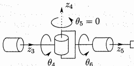
Figure 4.4: Spherical wrist singularity.
