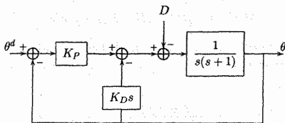
Figure 6.9: Second order system of Example 6.1 with PD Compensator.
