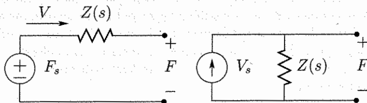
Figure 9.9: Thévenin and Norton equivalent networks.
