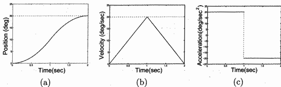
Figure 5.17: (a) Minimum-time trajectory. (b) Velocity profile for minimum-time trajectory. (c) Acceleration profile for minimum-time trajectory.
