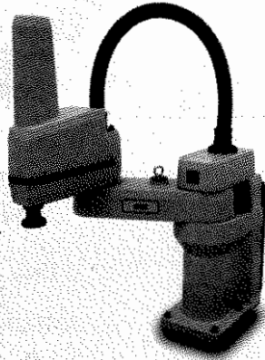
Figure 1.14: The Adept Cobra Smart600 SCARA Robot. The SCARA design is ideal for table top assembly, pick-and-place tasks, and certain types of packaging applications. (Photo Courtesy of Adept Technology, Inc.)
