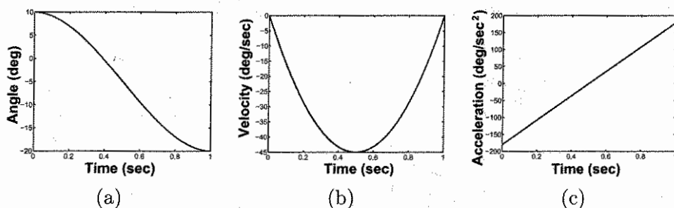
Figure 5.13: (a) Cubic polynomial trajectory. (b) Velocity profile for cubic polynomial trajectory. (c) Acceleration profile for cubic polynomial trajectory.
