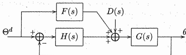
Figure 6.17: Feedforward control with disturbance D(s) .
