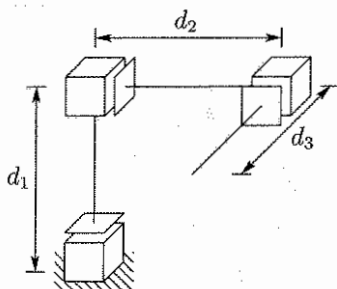
Figure 3.35: Cartesian configuration.
