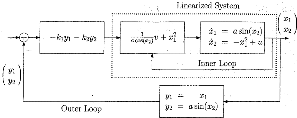
Figure 10.4: Inner-loop/outer-loop control architecture for feedback linearization.
