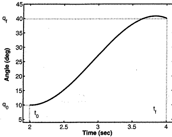
Figure 5.12: A typical joint space trajectory.
