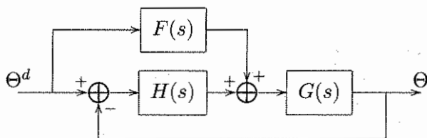
Figure 6.16: Feedforward control scheme. F(s) is the feedforward transfer function which has the reference signal \Theta^d as input. The output of the feedforward block is superimposed on the output of the compensator H(s) .
