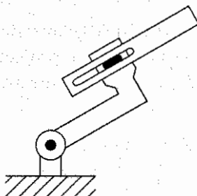
Figure 3.25: Two-link planar arm of Problem 3-4.
