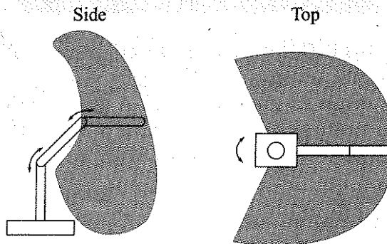
Figure 1.10: Workspace of the elbow manipulator. The elbow manipulator provides a larger workspace than other kinematic designs relative to its size.
