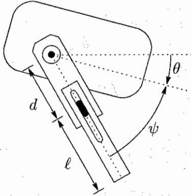
Figure 10.8: Hopping robot.
