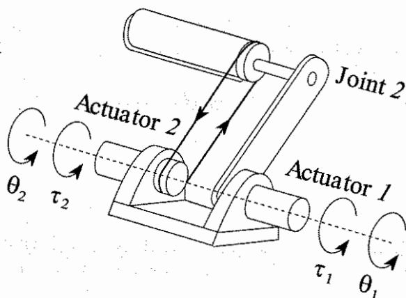
Figure 9.13: Two-link manipulator with remotely driven link.
