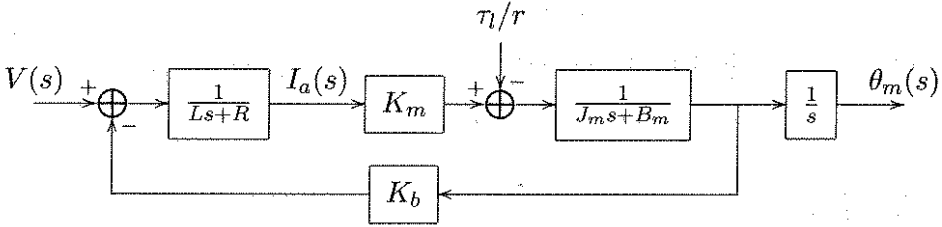
Figure 6.6: Block diagram for a DC motor system. The block diagram represents a third order system from input voltage V(s) to output position \theta_m(s) .
