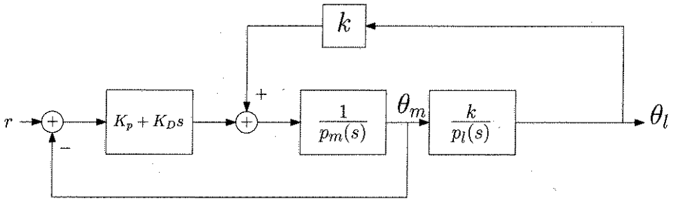
Figure 6.22: PD control with motor angle feedback.
