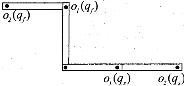
Figure 5.3: The initial configuration for the two-link arm is given by \theta_1 = \theta_2 = 0 and the final configuration is given by \theta_1 = \theta_2 = \pi/2 . The origins for DH frames 1 and 2 are shown at both q_s and q_f .
